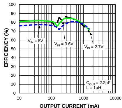
Efficiency ( V_{OUT} = 1.0V ) vs. Output Current
