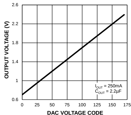
Output Voltage vs. DAC Linearity
